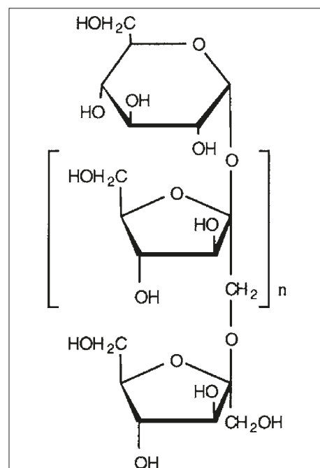
Figure 1. Chemical formula of an inulin
