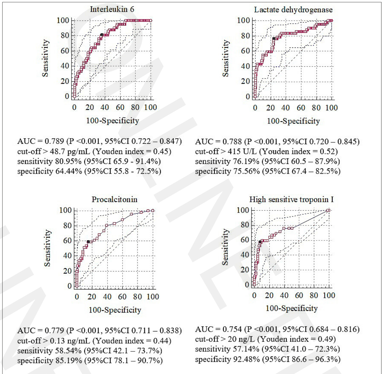
Figure 1. Receiver operating characteristic (ROC) curves for predictors with highest predictive value in univariate analysis
